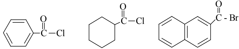
Benzoilxlorid Tsikloheksankarbonil- xlorid 2-Naftoilbromid
